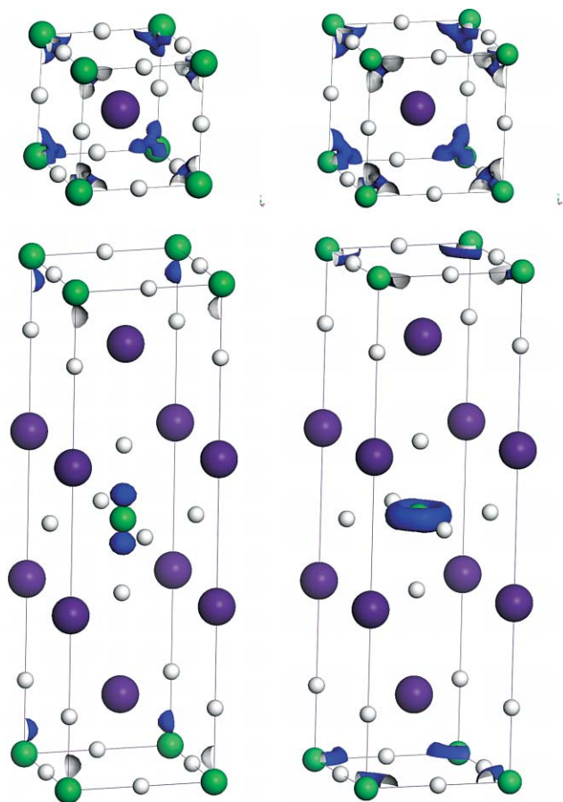
Fig. 2 Electronic density (in blue) at the Fermi level ( E_F \pm 0.03 eV) for CsYbH 3 (upper left), CsTmH 3 (upper right), Cs 2 YbH 4 (lower left) and Cs 2 TmH 4 (lower right). Density isovalue 0.012 e Å -3 .
