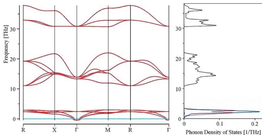
Fig. 3 Phonon band structure (left) and phonon DOS (right) for CsYbH 3 ; PHONON/VASP calculation. H’s contribution to phonon DOS is in black, Yb’s one in red, Cs’s one in blue.
