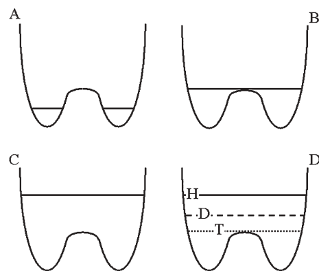
Fig. 4 The double-well PES for a mixed-valence compound for three different zero-point vibrational energy situations: (A) a separated (localized) mixed valence compound; (B) a fluctuating valence species; (C) an intermediate (delocalized) valence compound. Solid state analogues are likely to be (A) insulators, (B) superconductors, (C) ‘normal’ metals. Case (D) illustrates the postulated explanation for the inverse isotope effect observed experimentally for palladium hydride (PdH, PdD, PdT).
