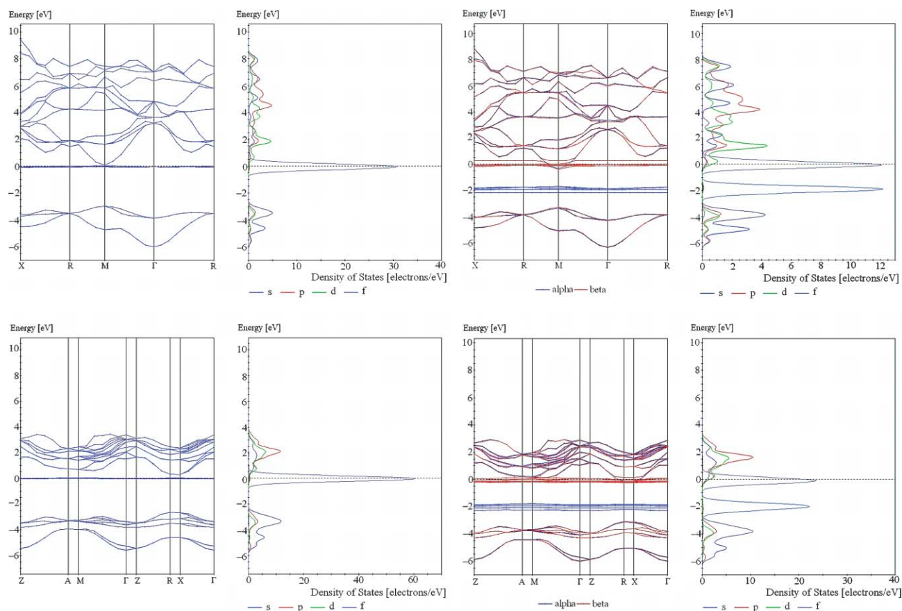
Fig. 1 Band structure and DOS for CsYbH 3 (upper left), CsTmH 3 (upper right), Cs 2 YbH 4 (lower left) and Cs 2 TmH 4 (lower right). Focus is on hydride, f and conduction bands.
