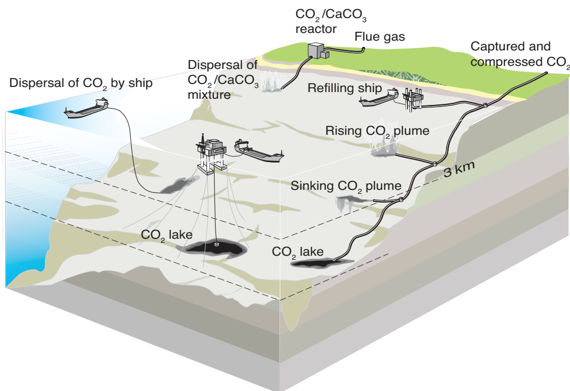
Figure TS.9. Methods of ocean storage.
