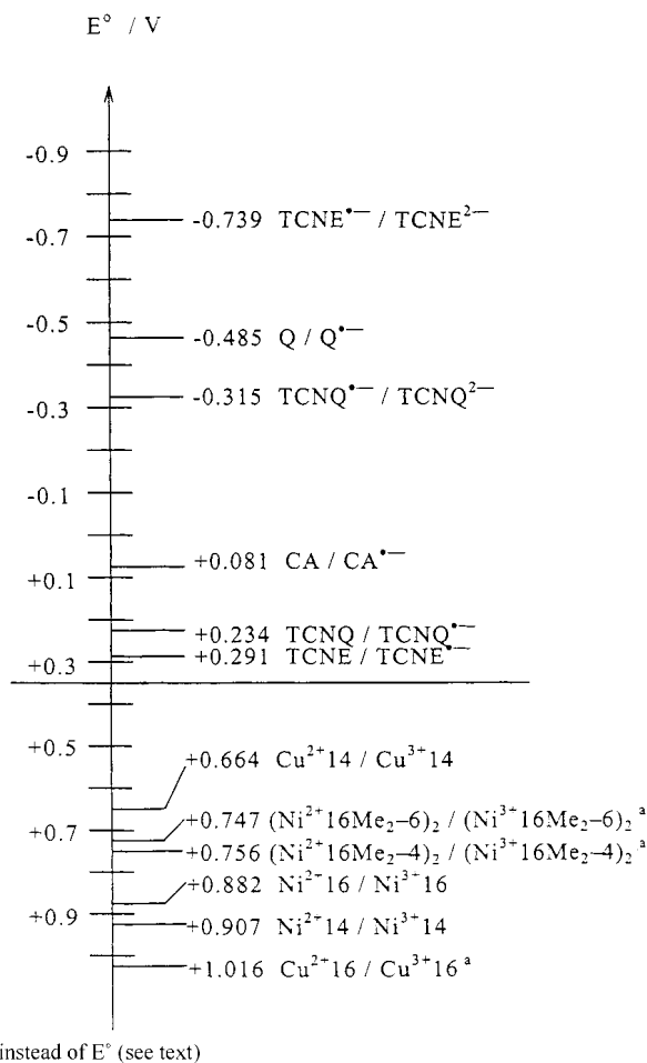
Figure 8. Positioning of the donors and acceptors under investigation in the common electric redox potential scale ( E in volts). The potentials were measured under the same conditions: 0.1 M TBAP in AN, scan rate 0.05 \text{ V s}^{-1} . A promising donor–acceptor pair, candidate for the bistability effect (in AN), corresponds to a donor oxidation potential slightly lower than the acceptor reduction potential (e.g. Cu14 –TCNE or Cu14 –TCNQ)
