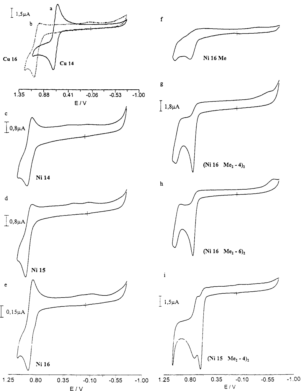
Figure 7. Redox properties of the tetraazaenemacrocylic complexes of \text{Cu}^{2+} and \text{Ni}^{2+} . CV curves for 0.4 mM Cu14 (a), Cu16 (b), Ni14 (c), Ni15 (d), Ni16 (e), Ni16Me (f), (Ni16Me 2 -4) 2 (g), (Ni16Me 2 -6) 2 (h) and (Ni15Me 2 -4) 2 (i) in 0.1 M a TBAP solution of acetonitrile, scan rate 0.05 V s -1 . The figure shows the oxidation potential dependence on the metal ion [(a) vs (c), (b) vs (e)], of the macrocycle size [(a) vs (b), (c) vs (d) and (e), (g) vs (i)] of the methyl substitution [(e) vs (f)], of the dimerization [(f) vs (g), (e) vs (g), (f) vs (h), (d) vs (i)] and of the bridge length [(g) vs (h)]. (a), (c) and (e) show the reversible oxidation processes. Note the cooperativity of oxidation in case (i).
